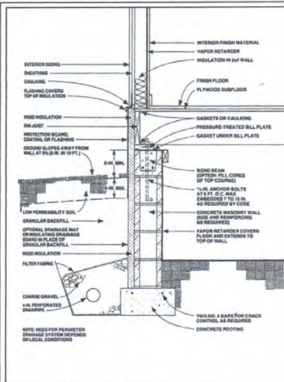
Research indicates that an insulated, unvented crawlspace can perform at least as well as a traditionally ventilated space. The detail, above, from DOE's Building Foundation Design Handbook, shows one option for an insulated crawlspace. The insulation can also go on the inside of the wall.
