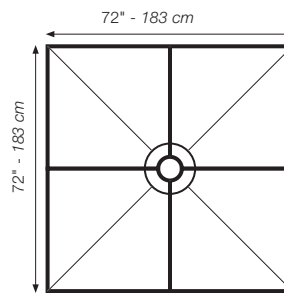
72" x 72" Kit - Select material for drain (ABS or PVC) and grate finish
