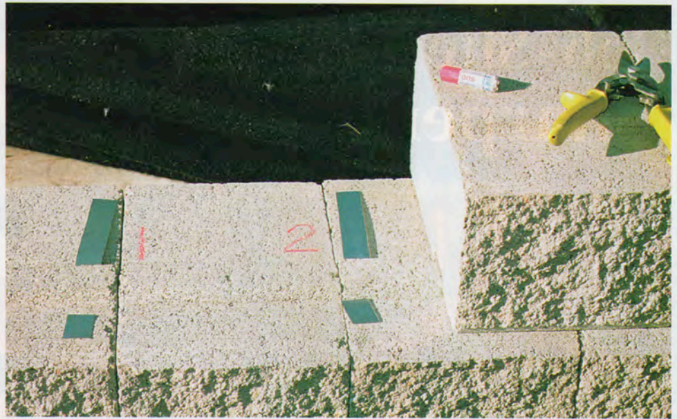
Weatherproof shims handle minor adjustments. For long stretches of wall, the author finds the work goes quickly (photo left). But slowdowns are inevitable. When the tops of adjacent blocks deviate by more than \frac{1}{32} in., adjustments may be required. When blocks have to be shimmed, the author uses narrow pieces of sheet aluminum that won't corrode, rot or wash away over time (photo above).
