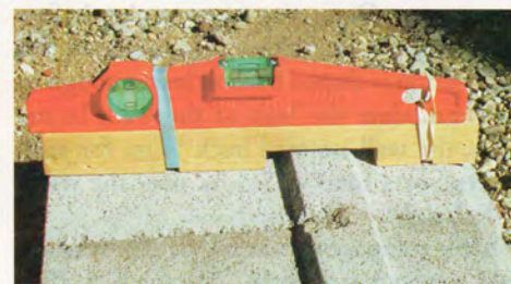
Modified for the job. A simple jig allows this torpedo level to straddle the lug cast into the top of each block so that it can be leveled front to back.
