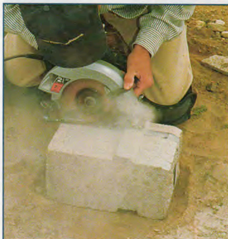
Cut block in three passes.
