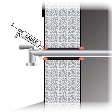
Figure 13.1. Caulk all plumbing penetrations through exterior walls.
