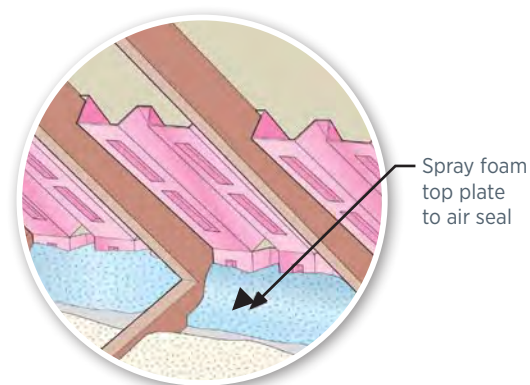
Figure 2.2. Pull back insulation to seal drywall to top plate with spray foam, caulk, or other sealer (Lstiburek 2010).
