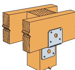
DJT14: Connects beams at the side of the post. ZMAX® coating or stainless steel recommended.
