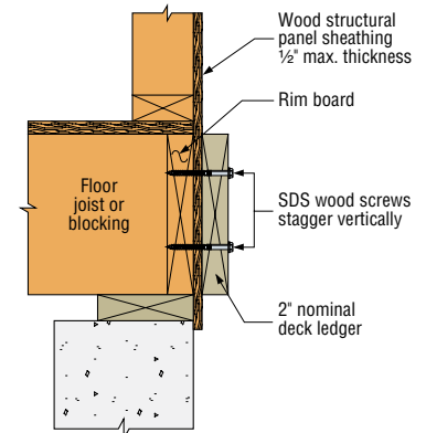
Ledger to rim board assembly
